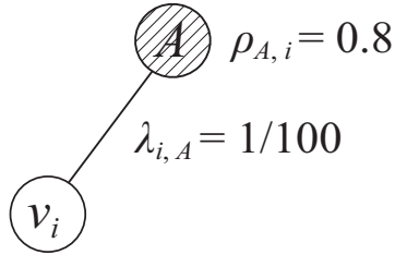
Figure 1: A contact graph.
