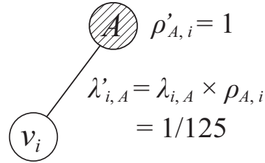
Figure 2: The reduced graph.
